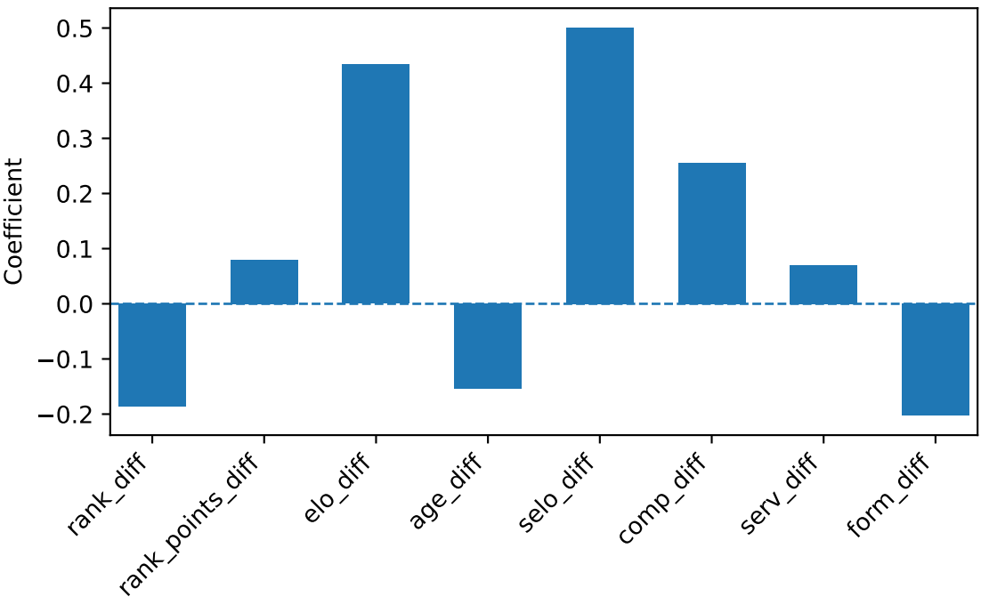
Average Logistic Regression Coefficients
